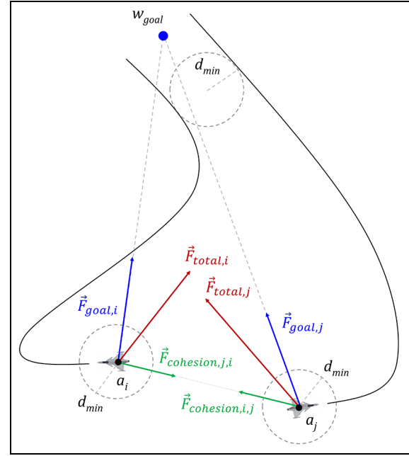
Figure 6. Gravitational grouping forces.
