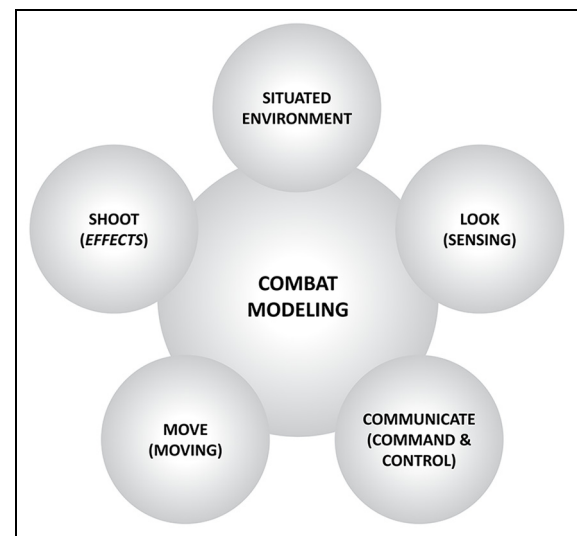
Figure 3. Combat modeling. 9
