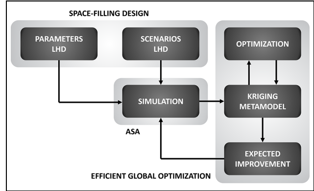
Figure 9. Adopted optimization strategy.
