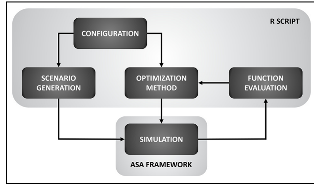
Figure 8. Conventional simulation optimization approach.
