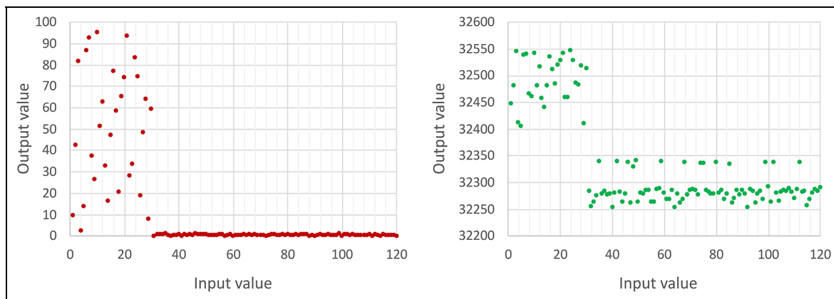
Figure 16. Distance-based with leader inputs (grouping value) and outputs (metric value) per simulation run.
