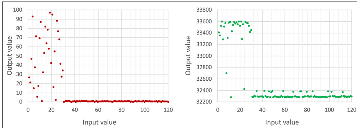
Figure 14. Distance-based leaderless inputs (grouping value) and outputs (metric value) per simulation run.
