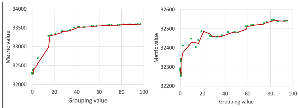
Figure 22. Moving average trendline for distance-based I/O data: leaderless (left) and with leader (right).
