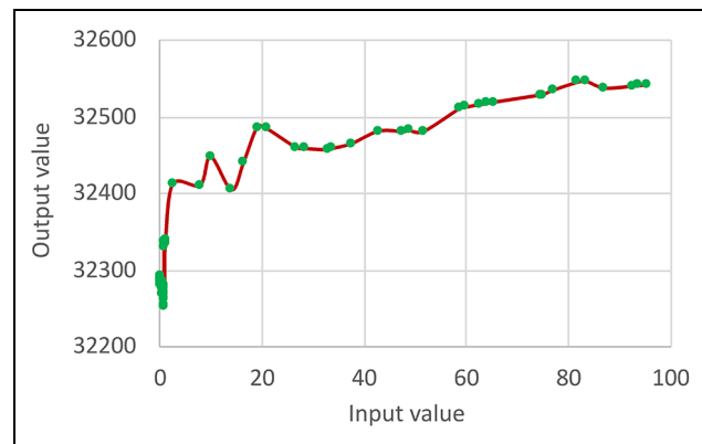
Figure 17. Distance-based with leader I/O data.
