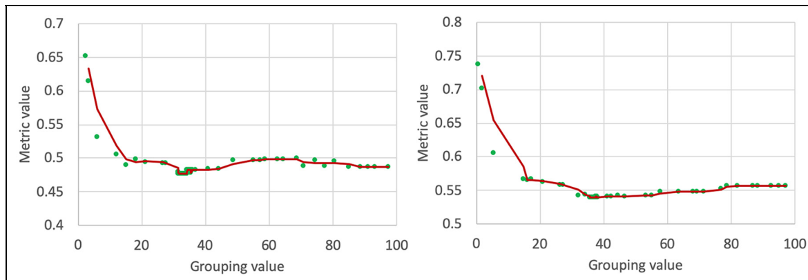
Figure 23. Moving average trendline for trajectory-based I/O data: leaderless (left) and with leader (right).
