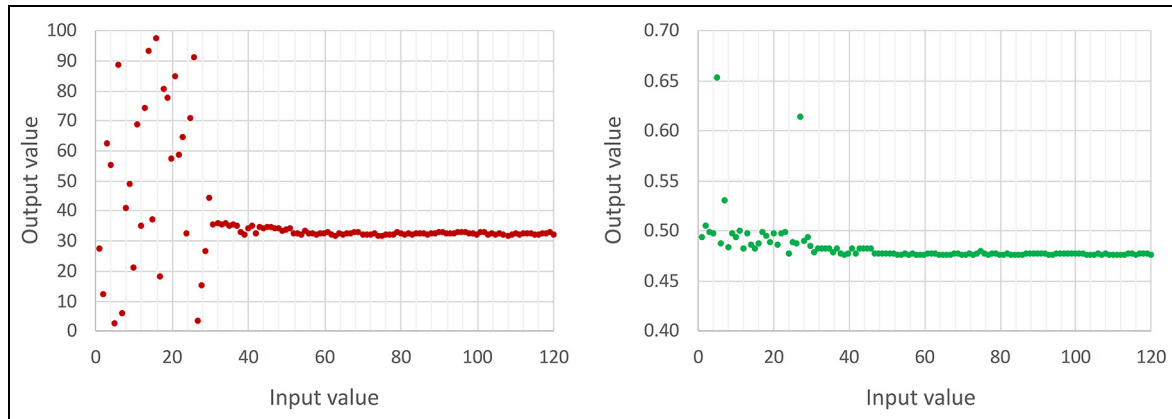
Figure 18. Trajectory-based leaderless inputs (grouping value) and outputs (metric value) per simulation run.
